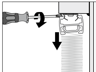
WANDWINKEL VS 7 / VS 8 CLIP PLAFOND / SUPPORT MURAL
