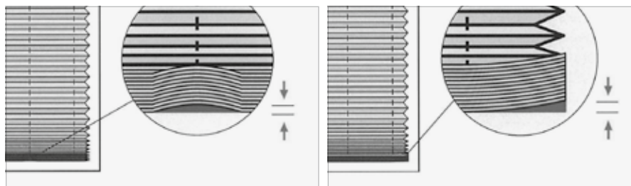
WAVINESS AT THE BOTTOM PROFILE The permissible tolerance range is 3 mm .
