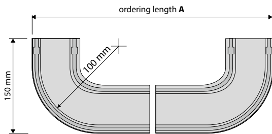
Return curve 4410/4420
