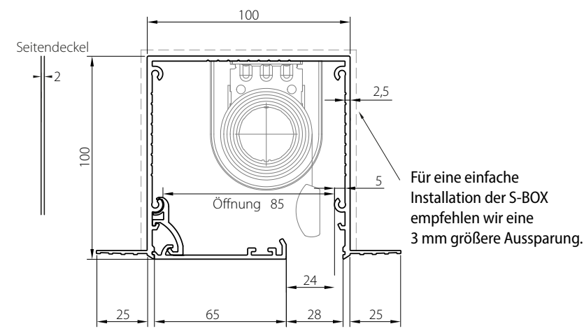
M-Basis
