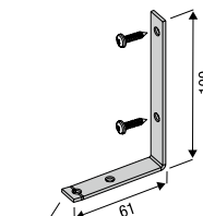
Montagewinkel wall fixing bracket support mural
