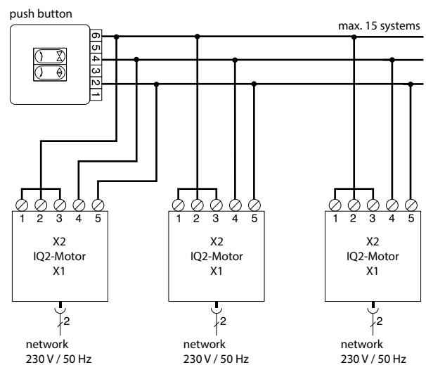
WIRING DIAGRAM
